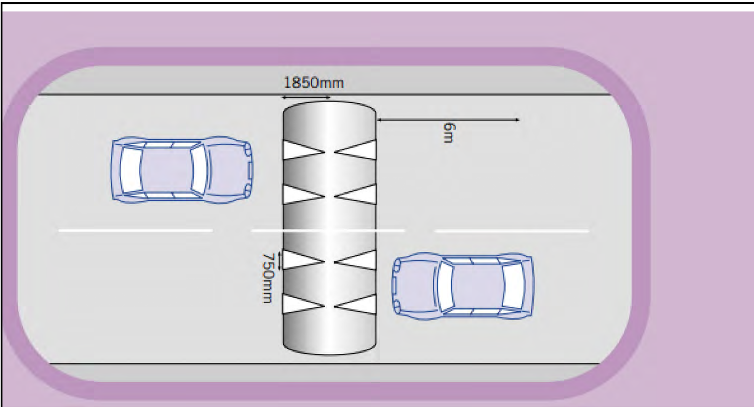
Proposed Round Top Ramp Detail
