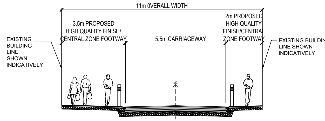
TYPICAL CROSS SECTION SECTION J-J
