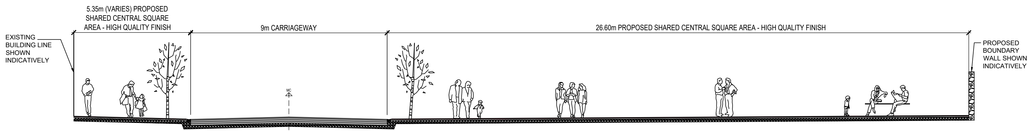
TYPICAL CROSS SECTION SECTION I-I
