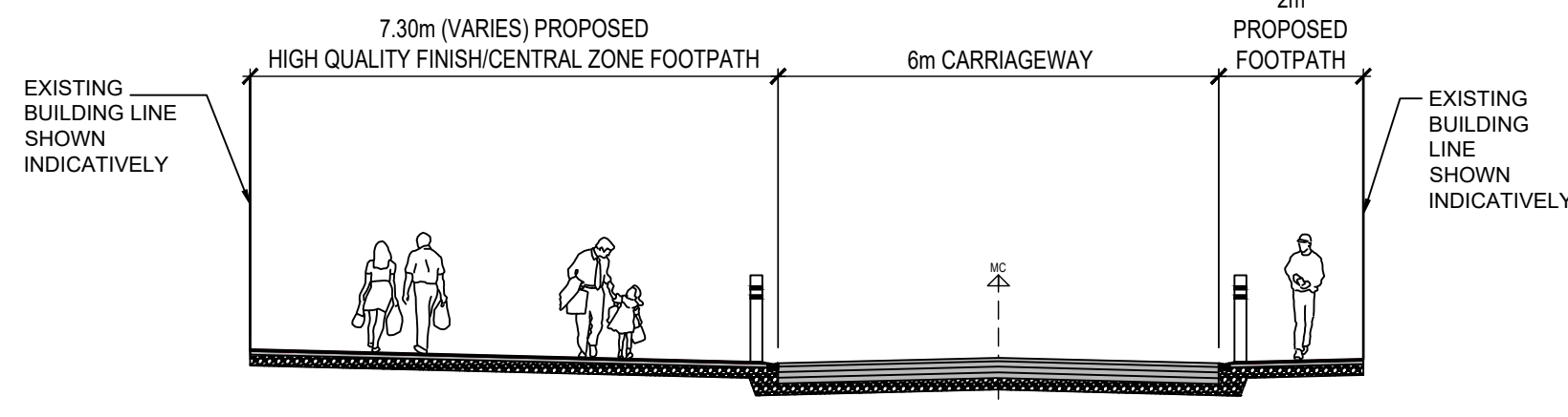
CROSS SECTION SECTION H-H
