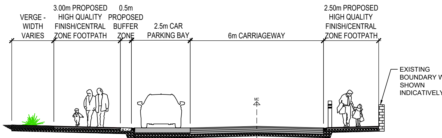
TYPICAL CROSS SECTION SECTION F-F
