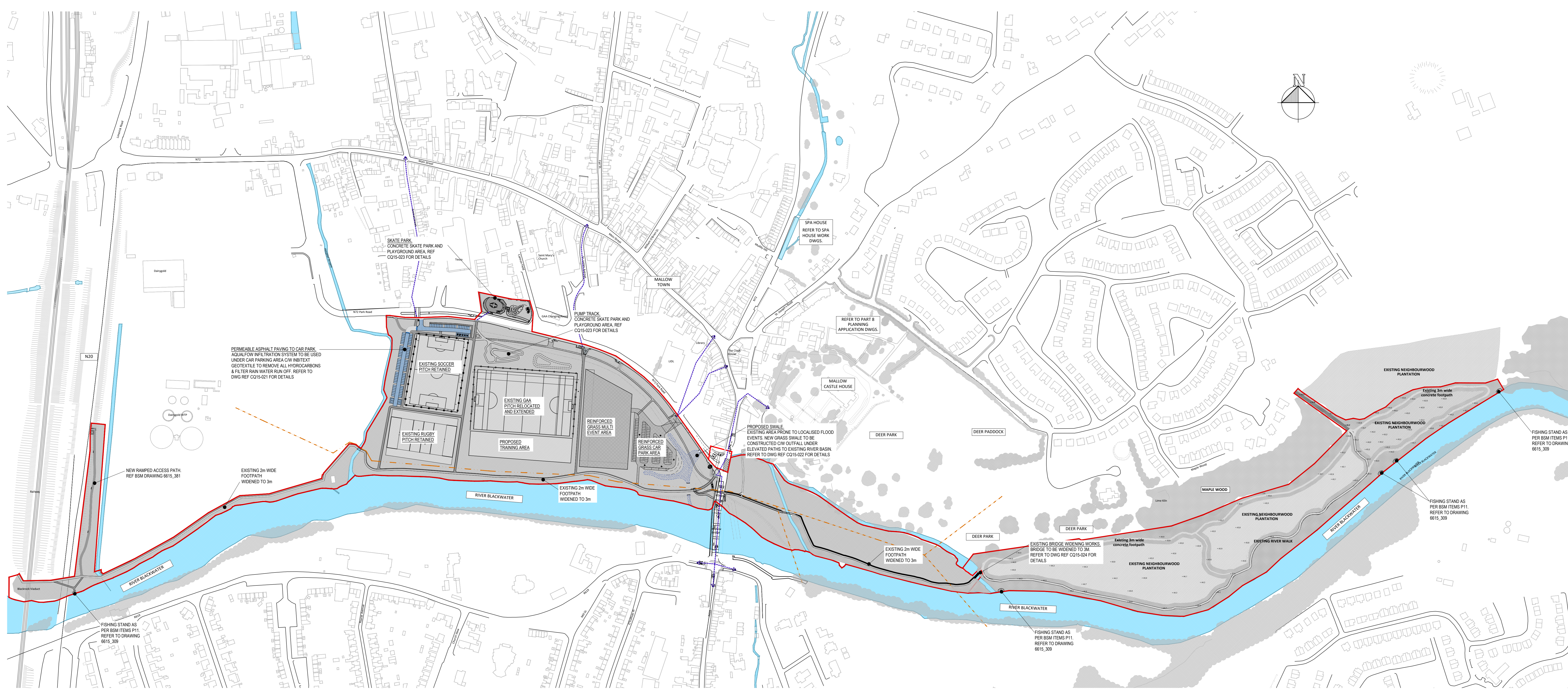
PROPOSED SITE LAYOUT PLAN SCALE 1:2500
