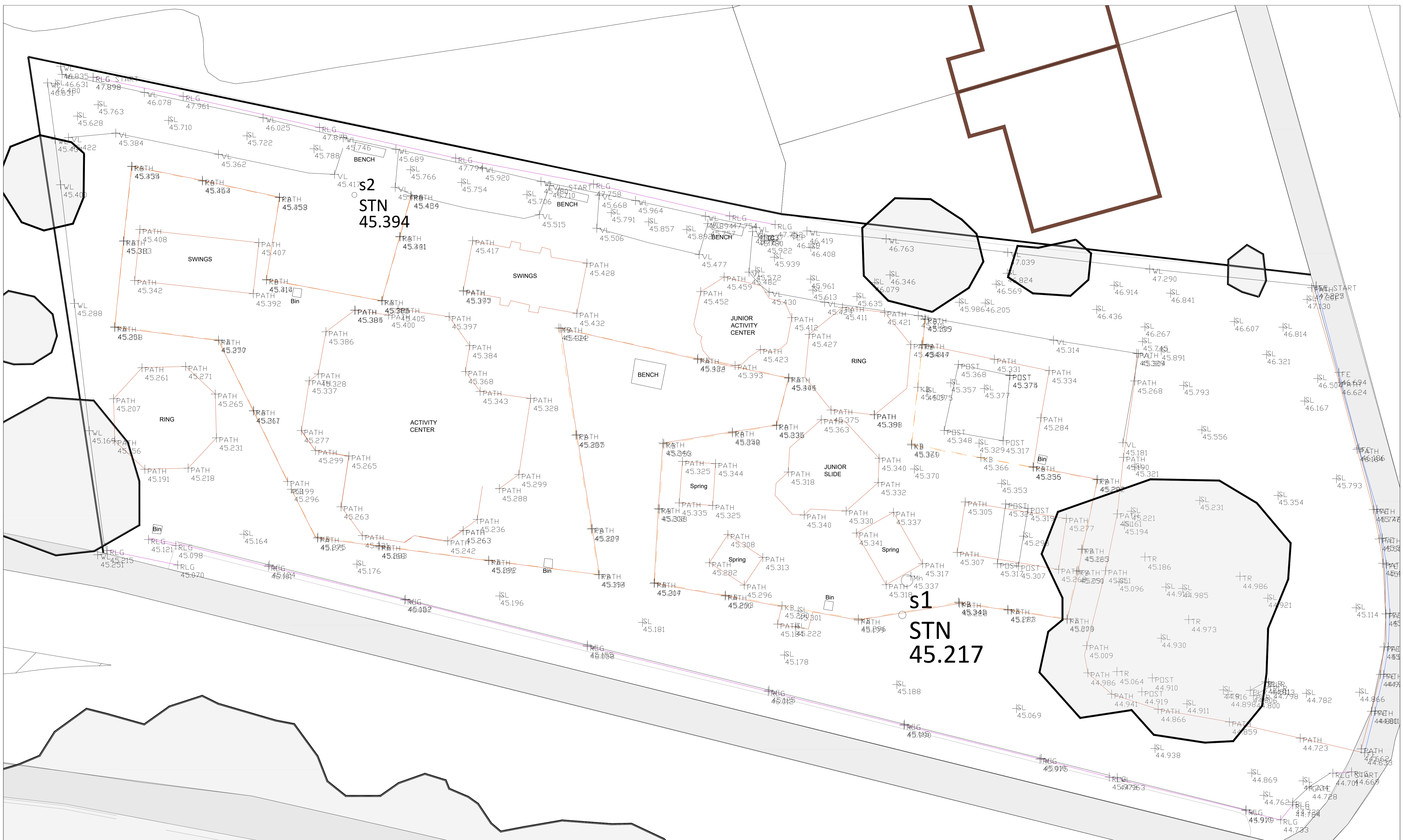
Existing Playground Survey Scale 1:100
