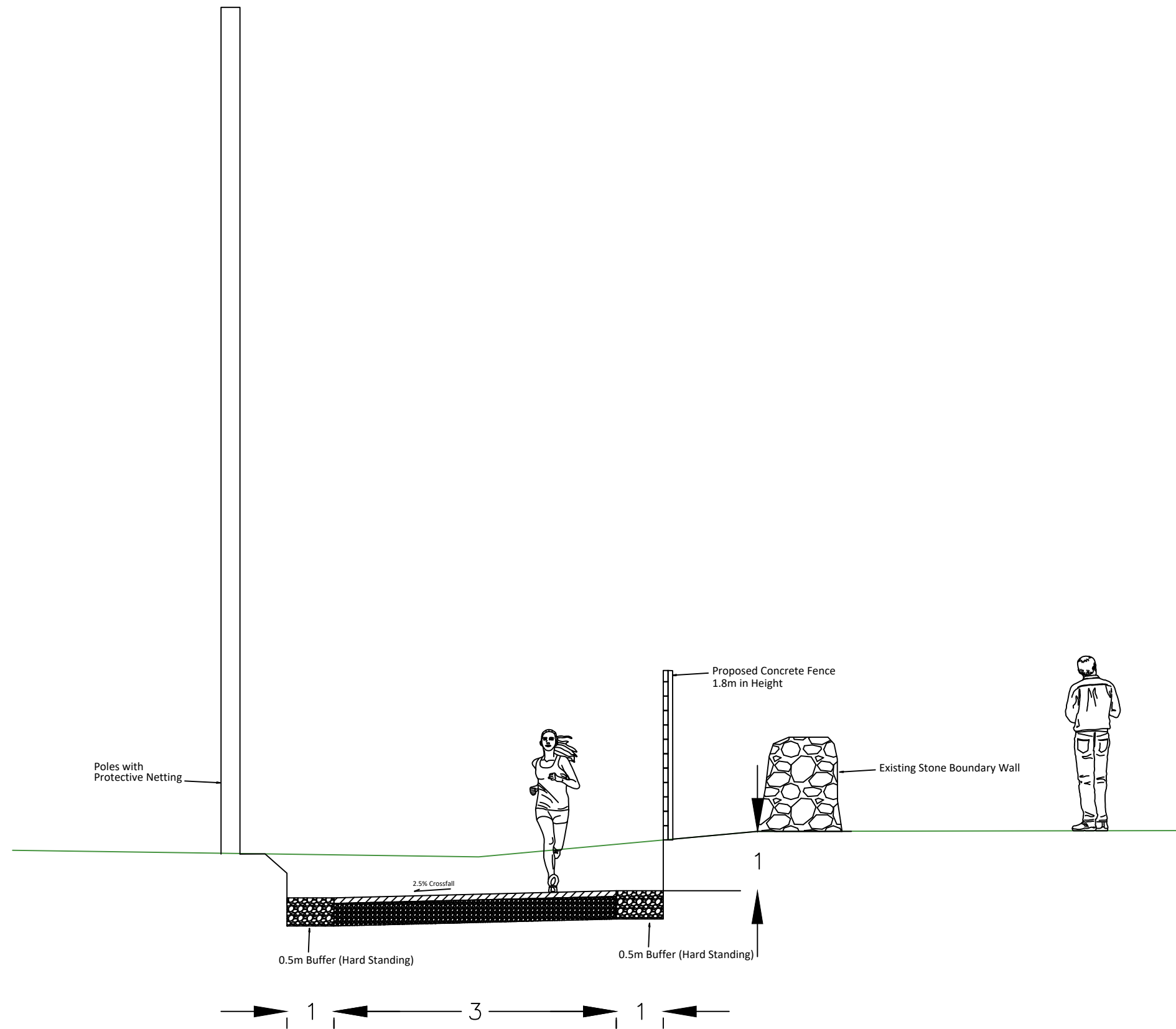
Section G2-G2
