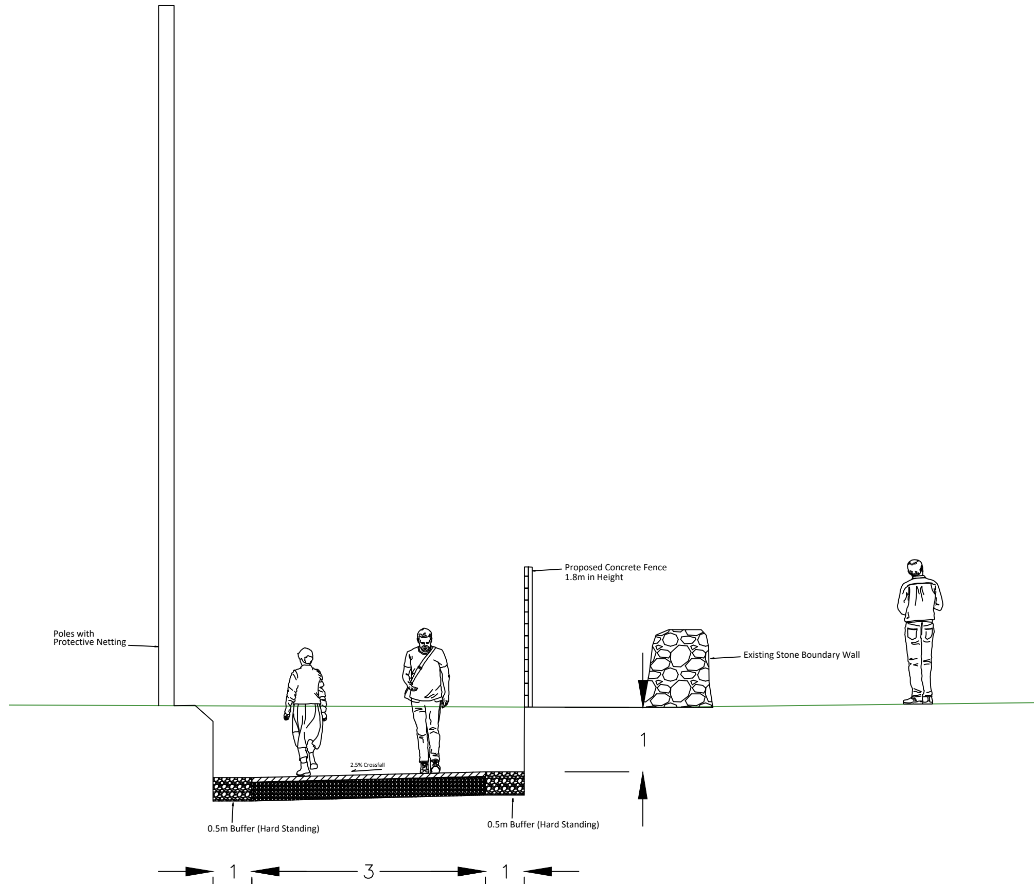
Section G1-G1
