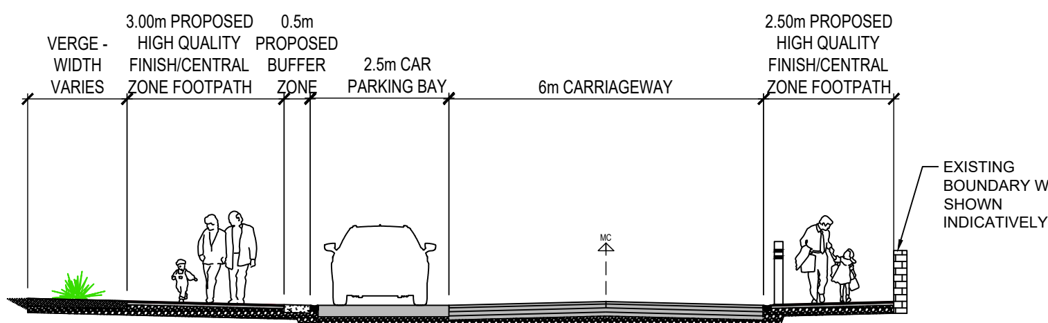
TYPICAL CROSS SECTION SECTION F-F
