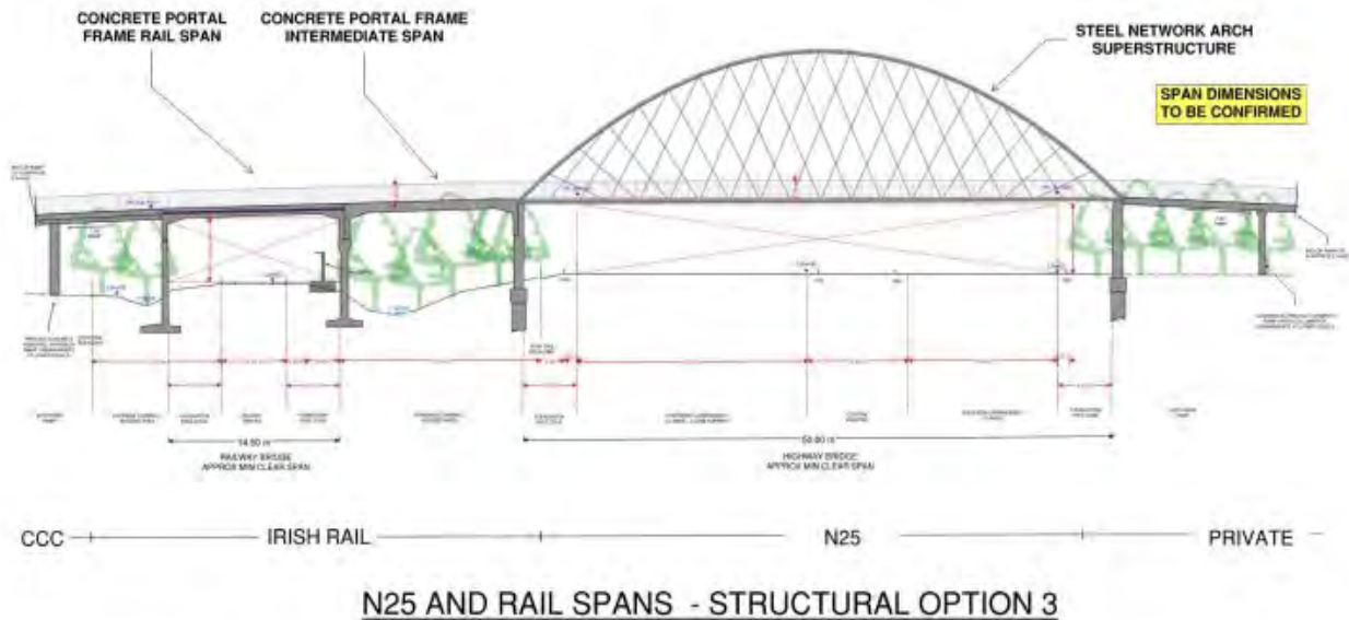
Image 3.3: Structural option 3
