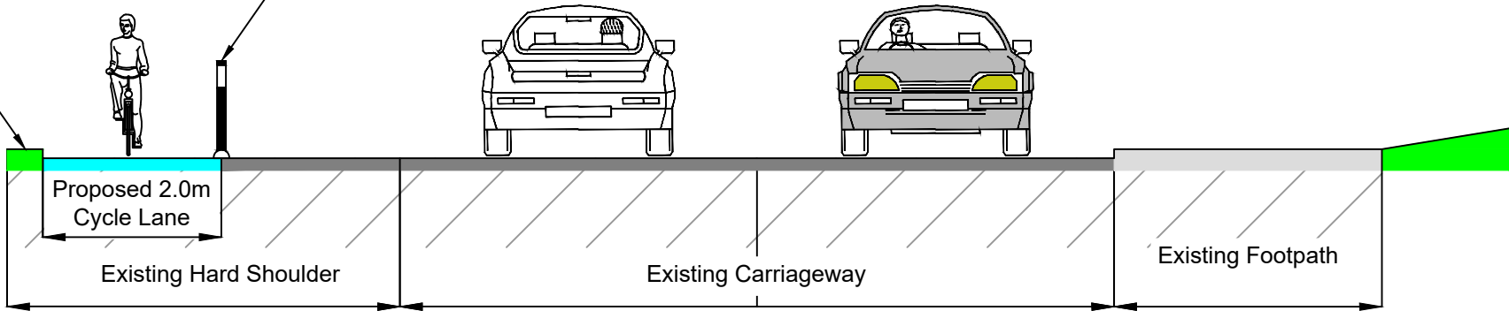
PROPOSED CROSS SECTION E-E (SCALE 1:75 @ A1, 1:150 @ A3)
