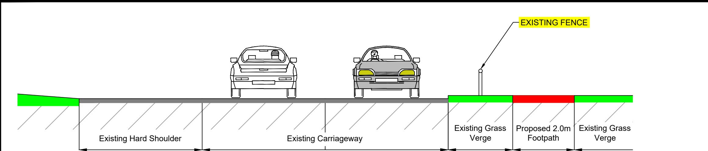
PROPOSED CROSS SECTION C-C (SCALE 1:75 @ A1, 1:150 @ A3)
